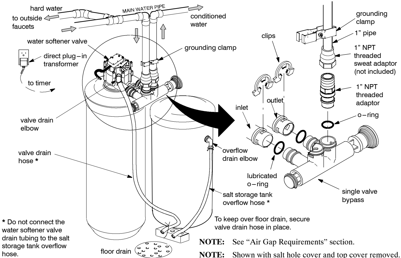
Figure 5 (typical installation)
