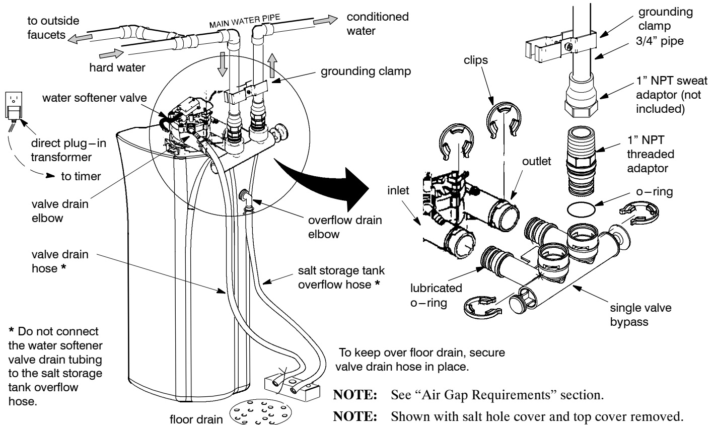
Figure 5 (typical installation)
