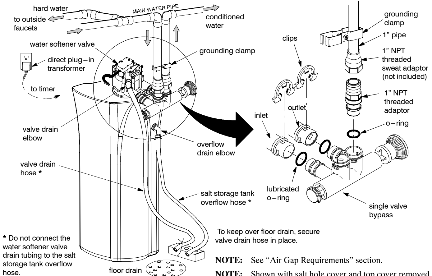
Figure 5 (typical installation)
